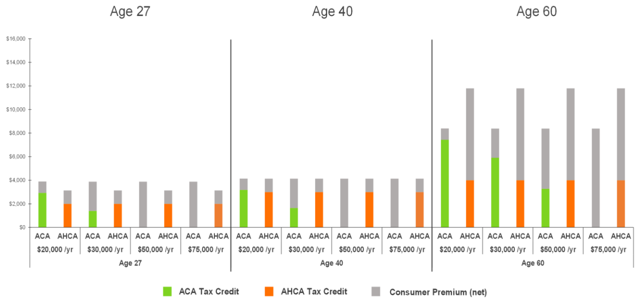
Figure 2b – Comparing Estimated ACA and AHCA Premiums and Tax Credits, by Age and Income, for a Low Cost Region (Salt Lake County), in 2020
